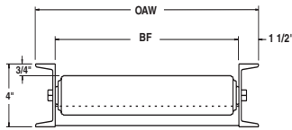
Single roller design
