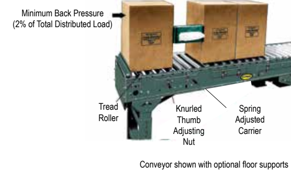
Conveyor shown with optional floor supports
